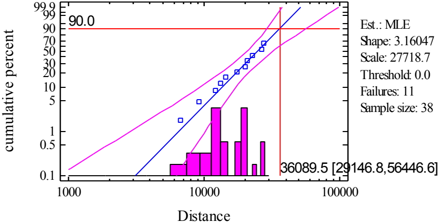
Weibull Plot
