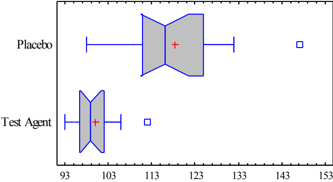
Box-and-Whisker Plot
