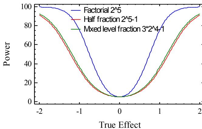
Power Curve
